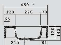
Basin ESCOCIA 1205 left MineralMarmo without bottle trap or clicker waste 1205 x 120 x 460 22683 | 736 €
