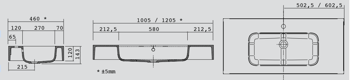
Basin ESCOCIA 1005 MineralMarmo without bottle trap or clicker waste 1005 x 120 x 460
