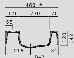
Basin ESCOCIA 1205 right MineralMarmo without bottle trap or clicker waste 1205 x 120 x 460 22684 | 736 €
