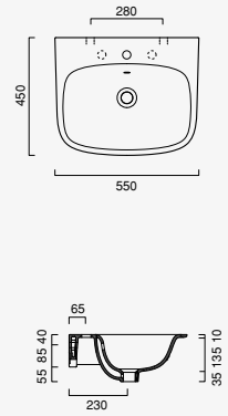
Green One 55 x 45 cod. 155GRON00
