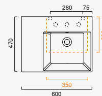
Premium Up 60 x 47 dx cod. 160DVPUP00
