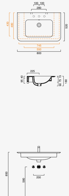
Green Up 80 x 52 cod. 180GRUP00
