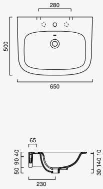
Green One 65 x 50 cod. 165GRON00
