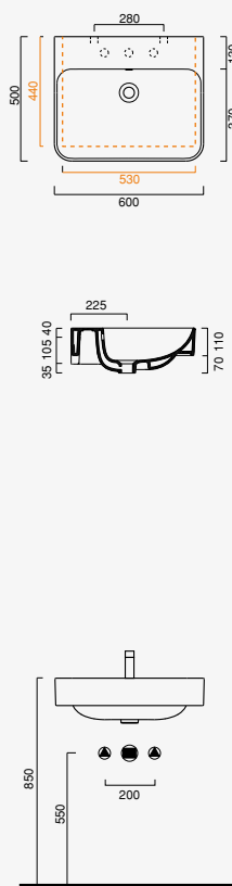
Green 60 x 50 cod. 160GR00
