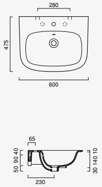
Green One 60 x 47.5 cod. 160GRON00
