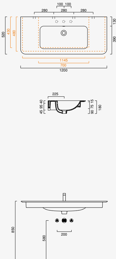
Green Up 120 x 52 cod. 1120GRUP00
