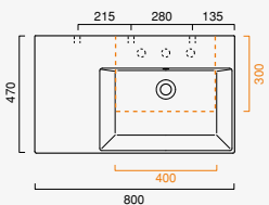
Premium Up 80 x 47 dx cod. 180DVP00
