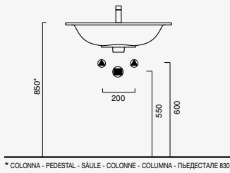
Green 60 x 38 cod. 160AGR00
