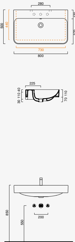
Green 80 x 50 cod. 180GR00
