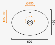
Velis 60 x 42 cod. 160VLN00
