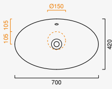
Velis 70 x 42 cod. 170VLN00
