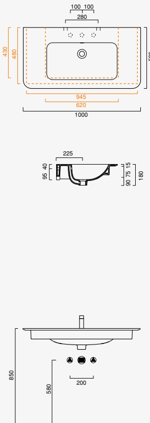
Green Up 100 x 52 cod. 1100GRUP00
