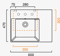
Premium Up 60 x 47 sx cod. 160SVPUP00
