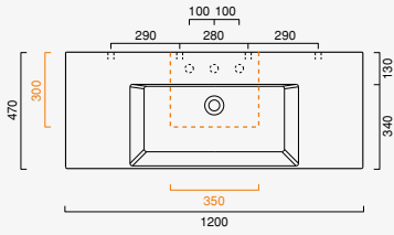
Premium Up 120 x 47 cod. 112VPUP00
