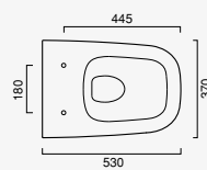
New Light wc Newflush® 53 cod. 1VSLIR00
