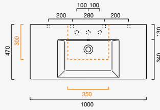
Premium Up 100 x 47 cod. 110VPUP00
