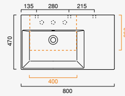
Premium Up 80 x 47 sx cod. 180SVP00
