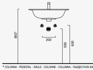
Green 50 x 38 cod. 150AGR00
