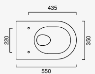
Zero wc Newflush® 55 cod. 1VS55NR00
