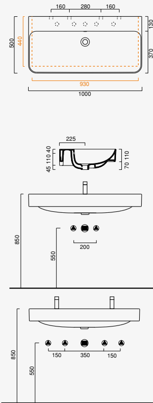
Green 100 x 50 cod. 1100GR00
